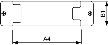
LCN8600/00 MultiOne interface USB2DALI
