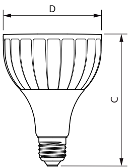
Master LED PAR30L 40W 30D 840
